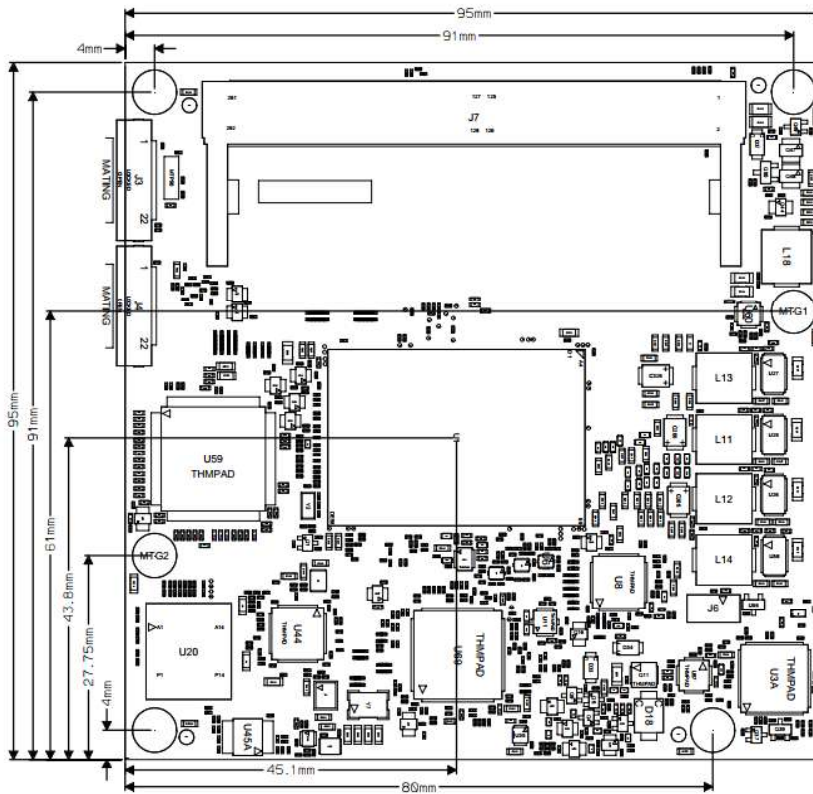
Figure 5: Module Dimensions
