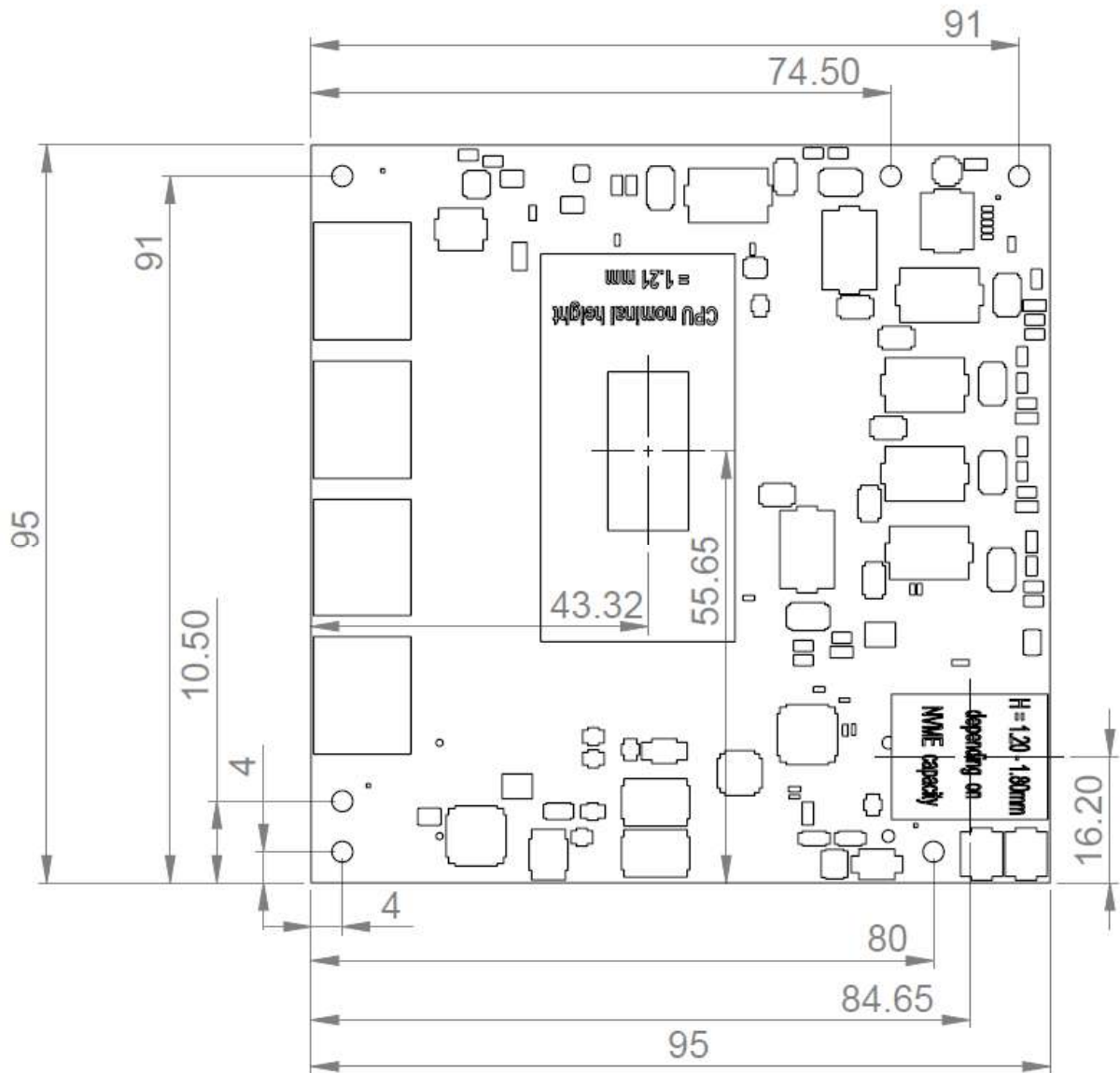
Figure 7: Module Dimensions
