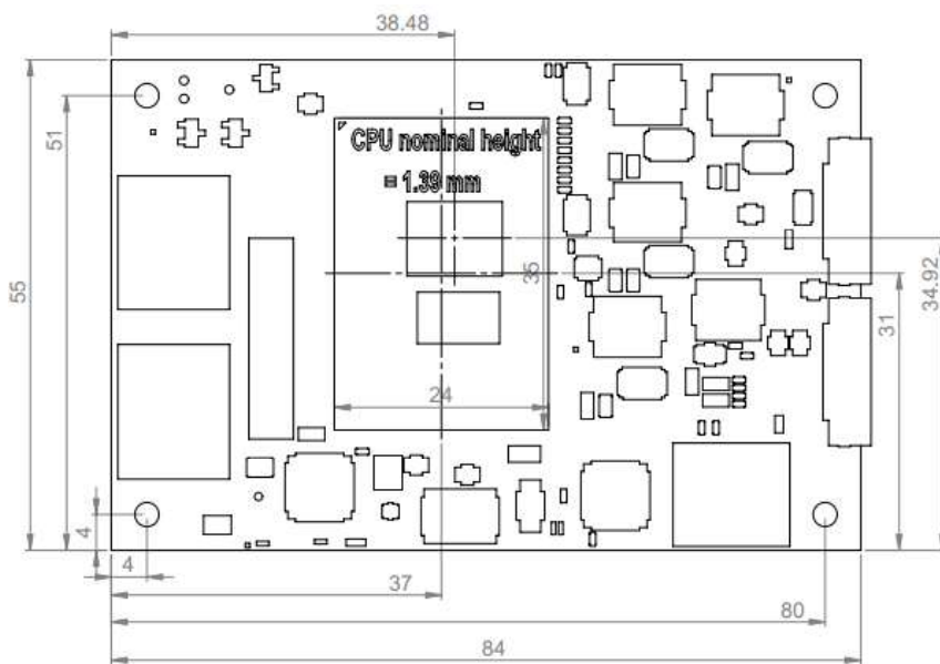
Figure 5: Module Dimensions
